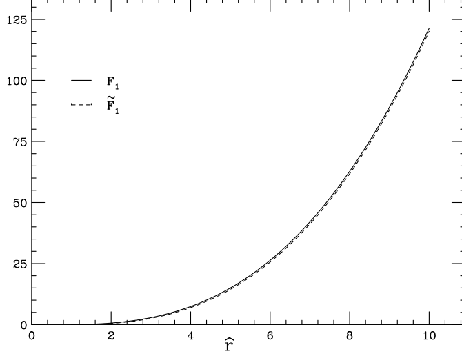
Figure 2: The functions F_1(\hat{r}) and \tilde{F}_1(\hat{r}) , defined in (2.21). Both functions are well-described by the approximation (3.4).
