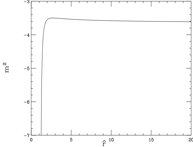
Figure 4: The mass that is defined in (3.9). It approaches the constant value -15/4 at large \hat{r} . The infinitely negative value at \hat{r} \rightarrow 1 gives rise to the Dirichlet boundary conditions (3.10).
