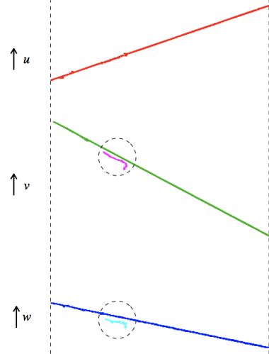
LongTracksTool
