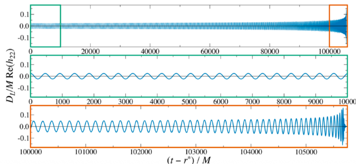
Figure. Example of NR simulation covering an 8 months signal with m_1/m_2 = 1/7 , \sim 10^6 CPU hours. It covers one point in parameter space. [Szilagyi et al. 2015]
