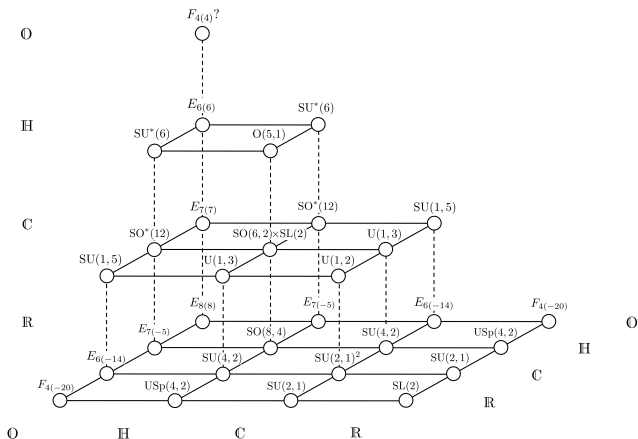
Figure: The conformal magic pyramid. Note, the exterior faces, up to real forms, are given by the magic square (i.e. the 4 \times 4 base) cut across its diagonal.
