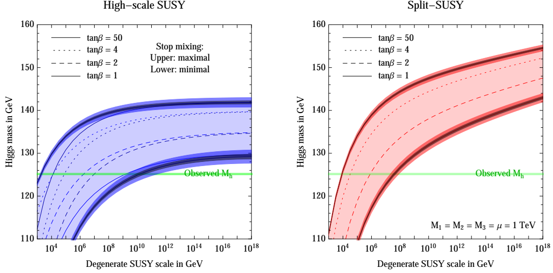
Figure 11: Higgs mass predictions as a function of the supersymmetry breaking soft mass scale and the Higgs sector parameter \tan\beta , taken from [66]. In the High-Scale scenario all soft masses \mu, \widetilde{M}_{1/2}, \widetilde{m}_0 are varied together, whereas in the Split SUSY scenario \mu, \widetilde{M}_{1/2} are kept at 1 TeV and only the scalar soft masses \widetilde{m}_0 are varied.
