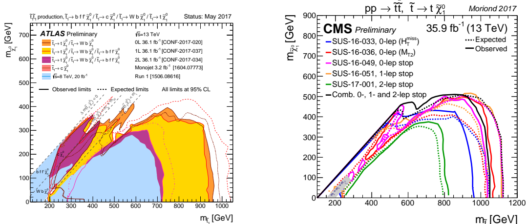
Figure 12: Current experimental limits on a simplified model with stop squarks and a neutralino. These limits are already placing significant pressure on SUSY naturalness for this class of models.
