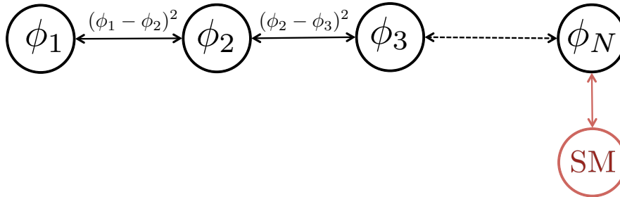
Figure 13: A schematic of dimensional deconstruction with a multi-site model. If some SM operator is coupled to the end of the chain it will inherit a suppressed coupling to the massless mode, scaling like 1/\sqrt{N} , as well as a coupling to the massive fields.
