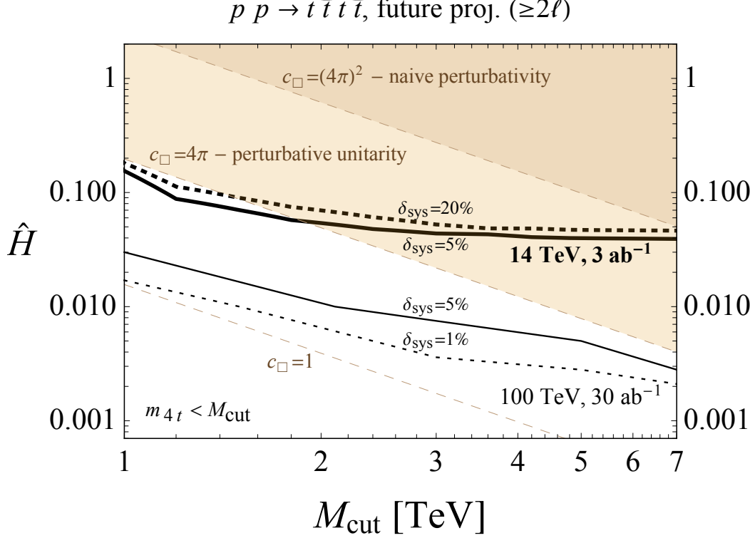
Figure 2: Projected constraints on \mathcal{O}_{\square} for given assumed values of the cutoff.
