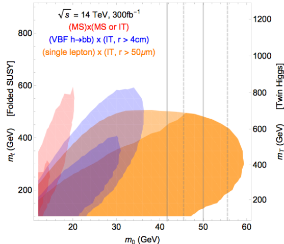
Figure 8: Expected collider limits on the parameter space of the Twin Higgs model (far right axes) from constraints on exotic Higgs decays. Figure taken from [29].
