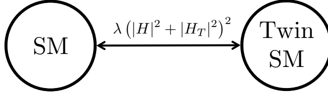
Figure 7: The structure of the Twin Higgs model. The SM and an entire copy are symmetric under a complete exchange of all fields. This ensures that the quadratic scalar action respects an accidental SU(4) symmetry, of which the SM Higgs is a pNGB. All interactions between the SM and Twin SM are through this single Higgs potential term.
