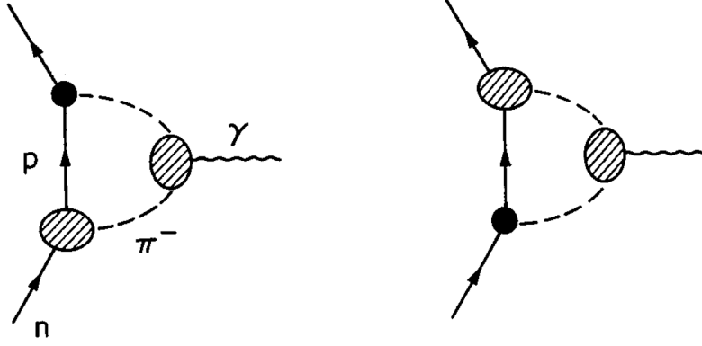
Figure 5: Generation of the neutron EDM from loops involving pions and the \eta' meson. Figure taken from the original CERN preprint [11].
