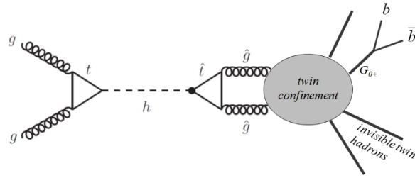
Figure 9: Twin glueball production and decay through the Higgs portal. Figure taken from [34].
