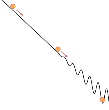
Figure 14: Evolution of the relaxion field in the early Universe from a point where the effective Higgs mass-squared is postive (left), passing through zero (middle), and negative (right).
