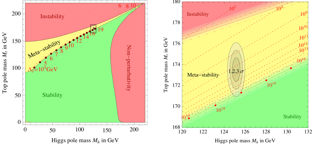
Figure 4: The Higgs vacuum structure, as a function of the weak-scale top and Higgs mass, in the SM, taken from [6].
