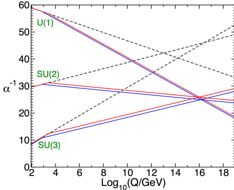
Figure 10: Renormalization group evolution of gauge couplings up to high energies, taken from [35]. The Standard Model gauge couplings are shown in dashed black and the gauge couplings with superpartners added, with masses in the range 0.75 \rightarrow 2.5 TeV, are shown in red and blue. Unification of the forces at high energies is clearly apparent in the supersymmetric case.
