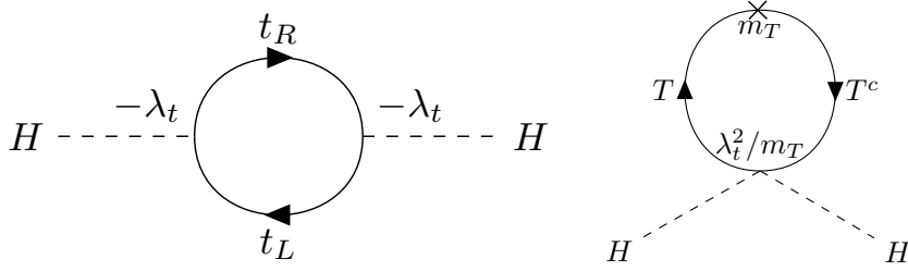
Figure 6: The cancellation between quadratic divergences from the top quark loop and fermionic top-partner loops.
